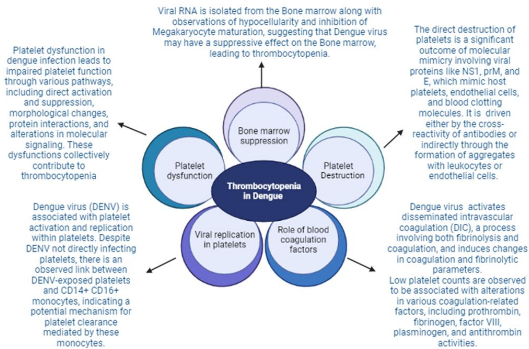
Figure 4: A summary of the development of thrombocytopenia in dengue due to the suppression of bone marrow, destruction and dysfunction of platelets, development of DIC, and viral replication in platelets: Adapted from, Dengue Fever: Therapeutic Potential of Carica Papaya L. Leaves, Sarker, Md.M.R., Khan, F. and Mohamed, I.N. (2021). Frontiers in Pharmacology , doi:https://doi.org/10.3389/fphar.2021.610912(62).
