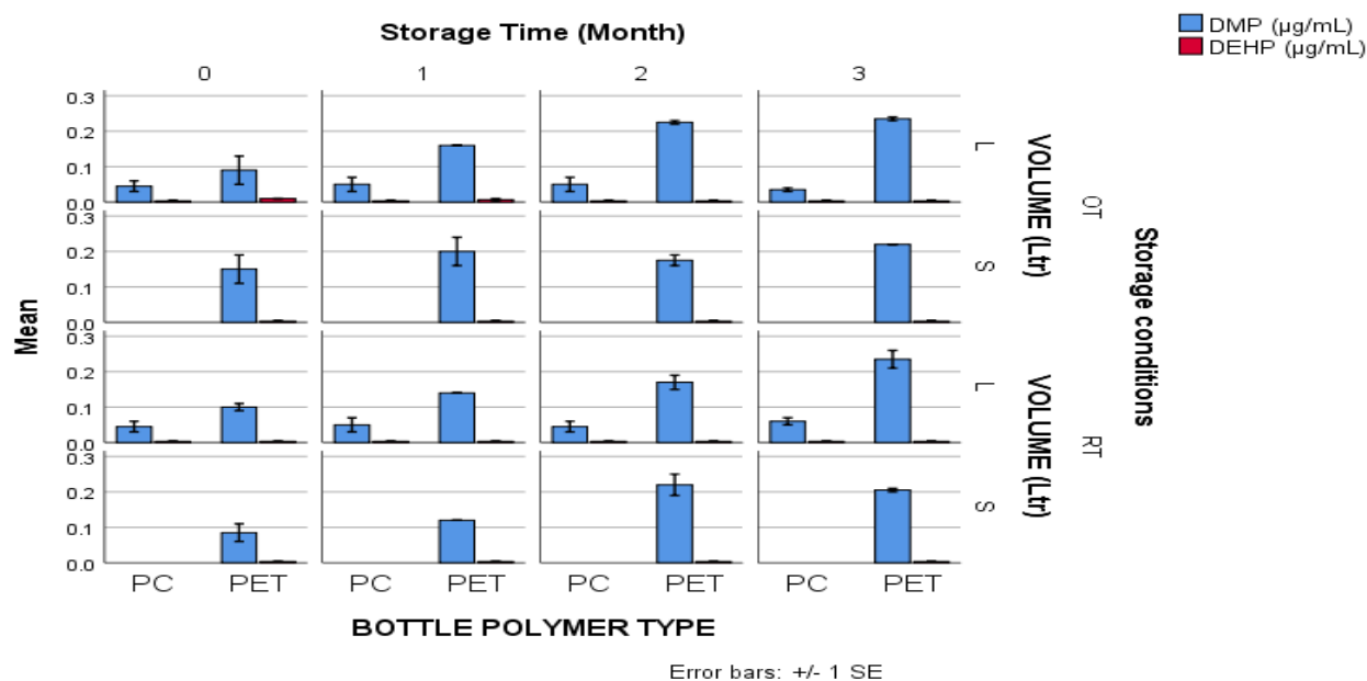
Figure 1: Mean concentrations of DMP and DEHP in \mu\text{g/mL} observed in PET and PC water samples were analysed at different times and under various storage conditions. Panel RT: storage at room temperature ( 25 \pm 5 °C); and Panel OT: storage outdoors with sun exposure ( 30 \pm 5 °C). The 0 storage time point denotes analysis before storages (2 weeks after production), whereas 1 denotes analysis 2 months, 2 denotes analysis 4 months, and 3 denotes analysis 6 months after storage. PET and PC denotes PET and PC bottles respectively while L and S denotes 18.9 ltr and 1.5ltr volumes of drinking water respectively.
