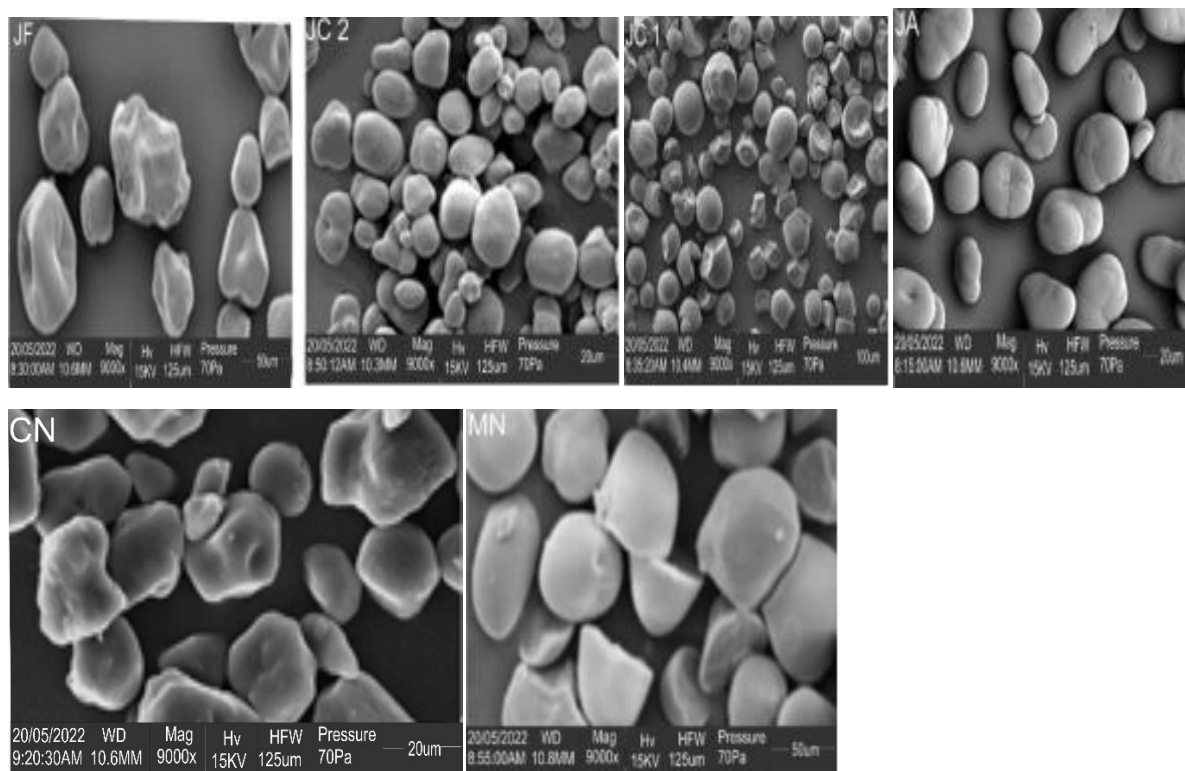
Fig. 4: SEM Image of the starch samples at 9000x magnifications
