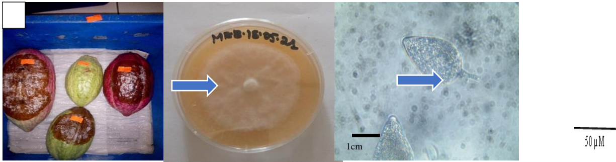
Fig. 2: Culture of P. megakarya and observation of its sporangiospores (A: Necrotic cocoa pods, B: Clusters of mycelium in a Petri dish, C: Sporangiospores)
