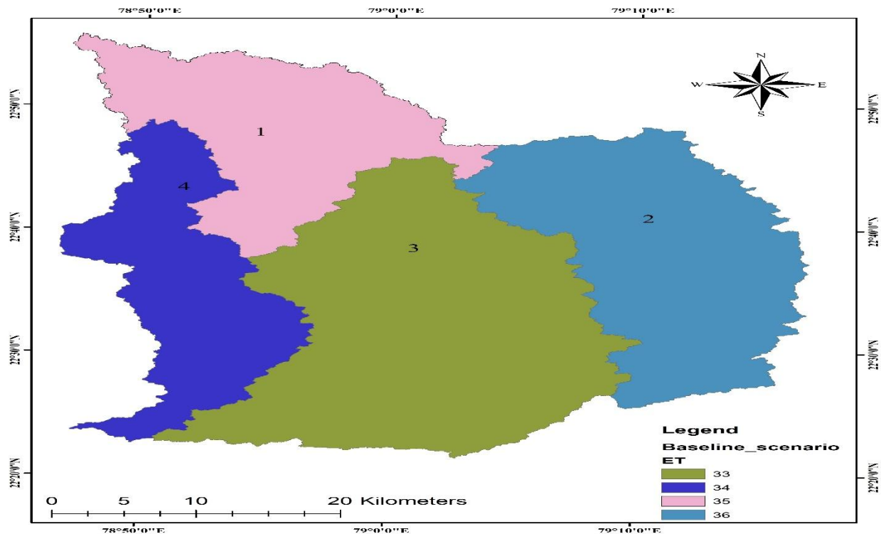
Fig.3 Spatial variation of the ET in the Gadawara watershed
