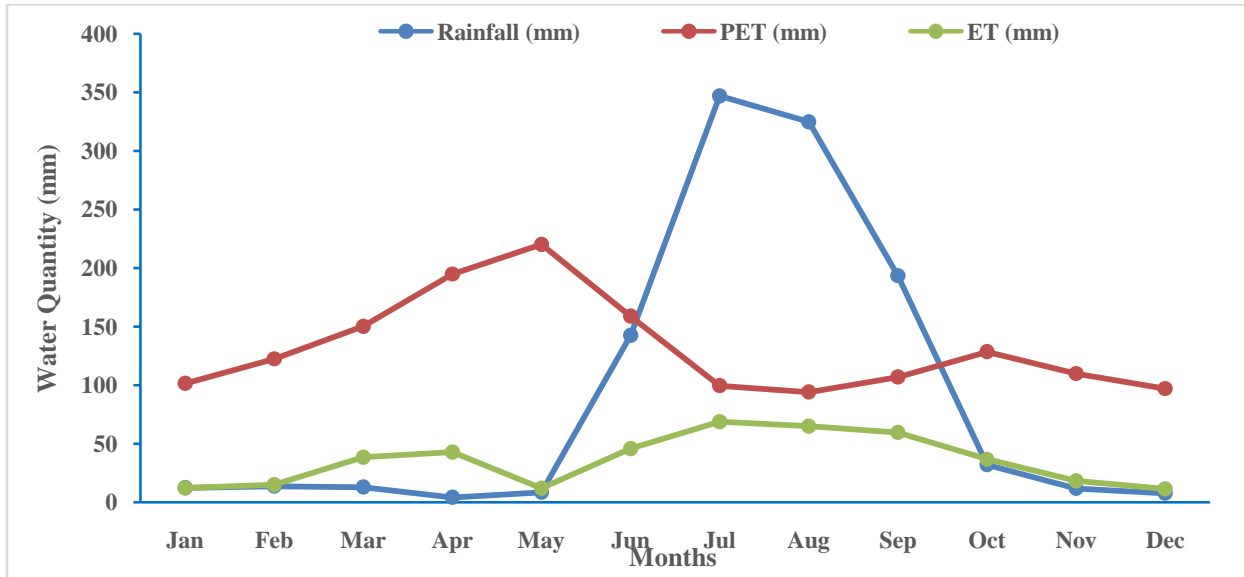
Fig.5 Average monthly Rainfall, PET and ET of Gadarwara watershed
