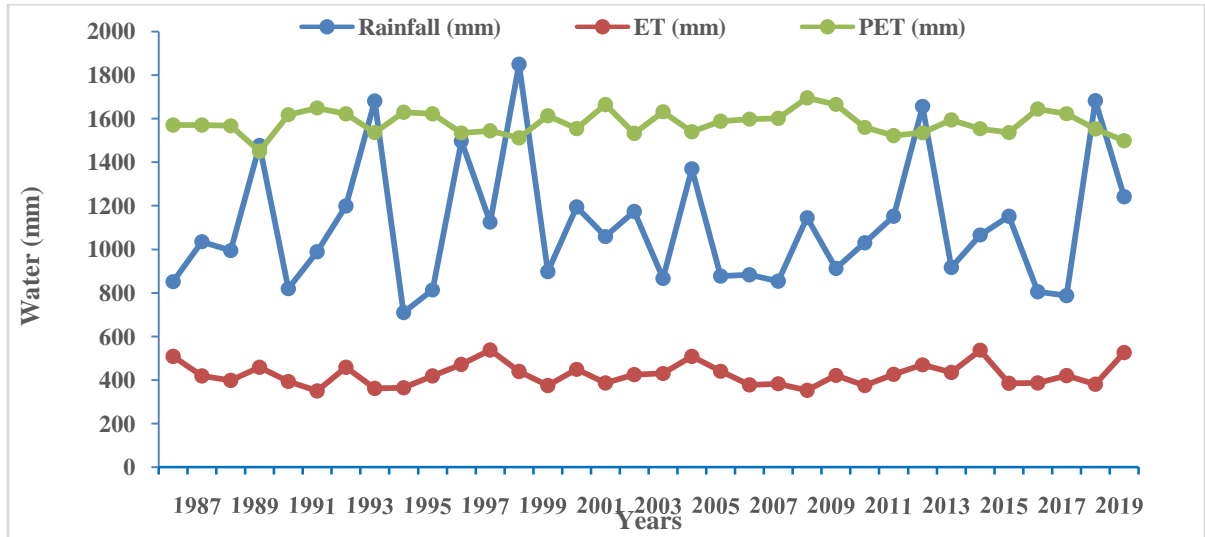
Fig.4 Yearly Rainfall, PET and ET of Gadarwara watershed
