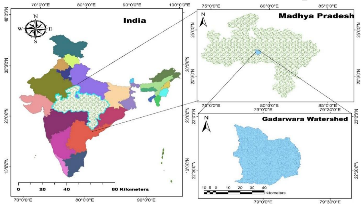
Fig.1 Map of Gadarwara Watershed
