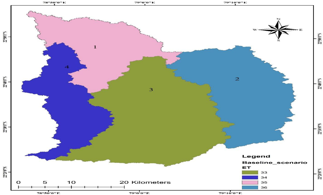
Fig.3 Spatial variation of the ET in the Gadarwara watershed
