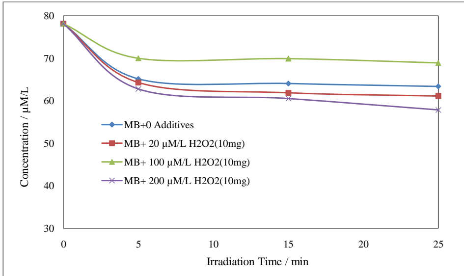
Fig. 5a: Effect of 10 mg of H 2 O 2 (10mg) on the degradation of MB
