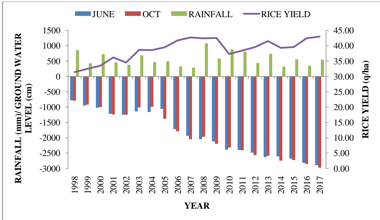
Fig. 5 Relationship of monsoon rainfall with groundwater level and rice productivity at Patiala
