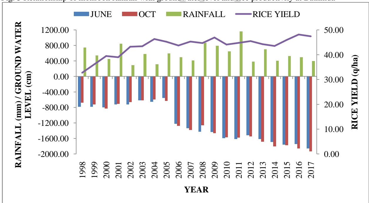
Fig. 4 Relationship of monsoon rainfall with groundwater level and rice productivity at Ludhiana
