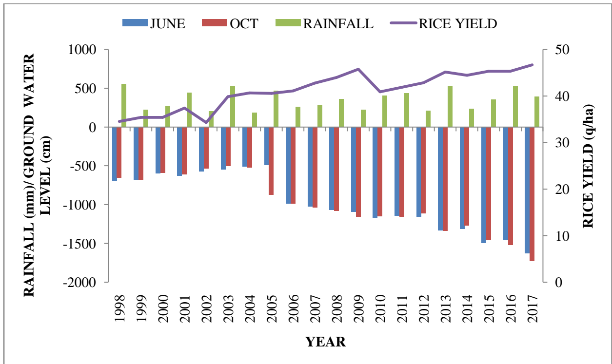
Fig. 3 Relationship of monsoon rainfall with groundwater level and rice productivity at Bathinda
