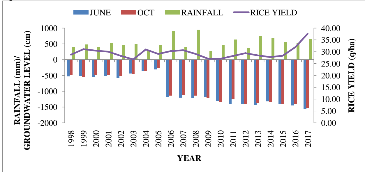
Fig. 1 Relationship of monsoon rainfall with groundwater level and rice productivity at Amritsar
