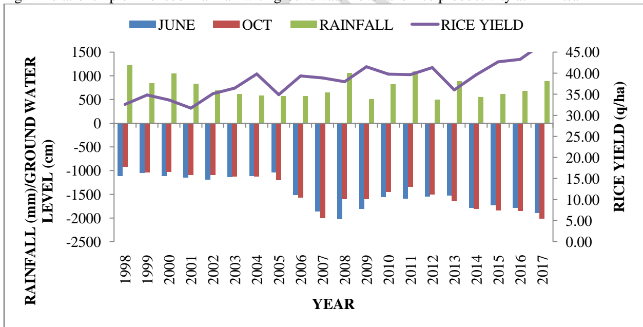
Fig. 2 Relationship of monsoon rainfall with groundwater level and rice productivity at BallowalSaunkhri
