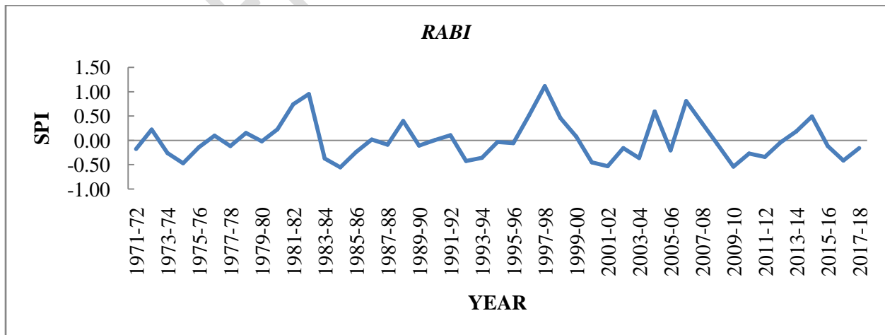
Fig.3 Standardized precipitation index at Bathinda (Annual, Kharif and Rabi)
