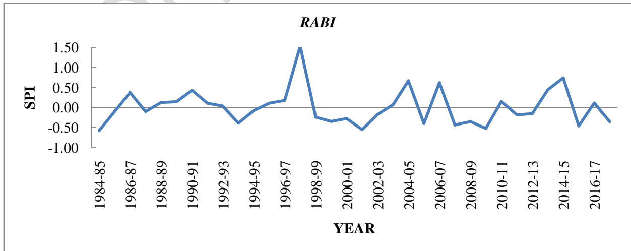
Fig.2 Standardized precipitation index at BallawalSaunkhri (Annual, Kharif and Rabi)
