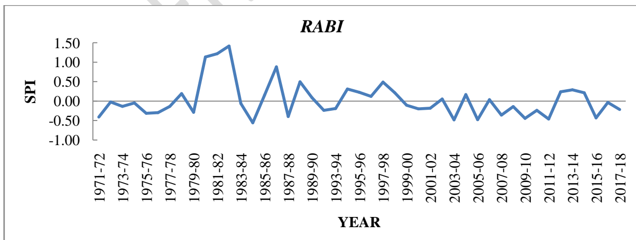
Fig. 5 Standardized precipitation index at Patiala (Annual, Kharif and Rabi)
