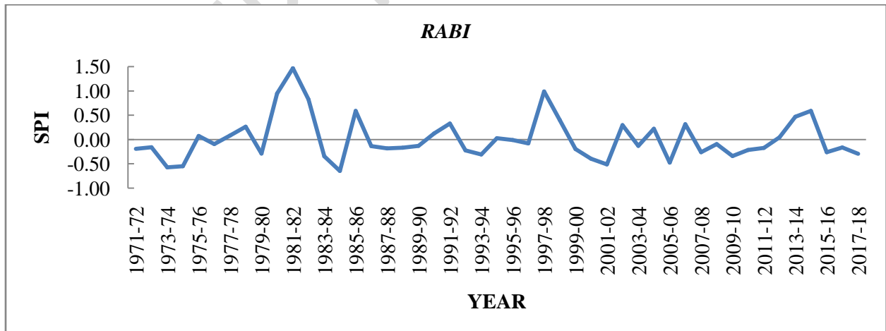
Fig.4 Standardized precipitation index at Ludhiana (Annual, Kharif and Rabi)
