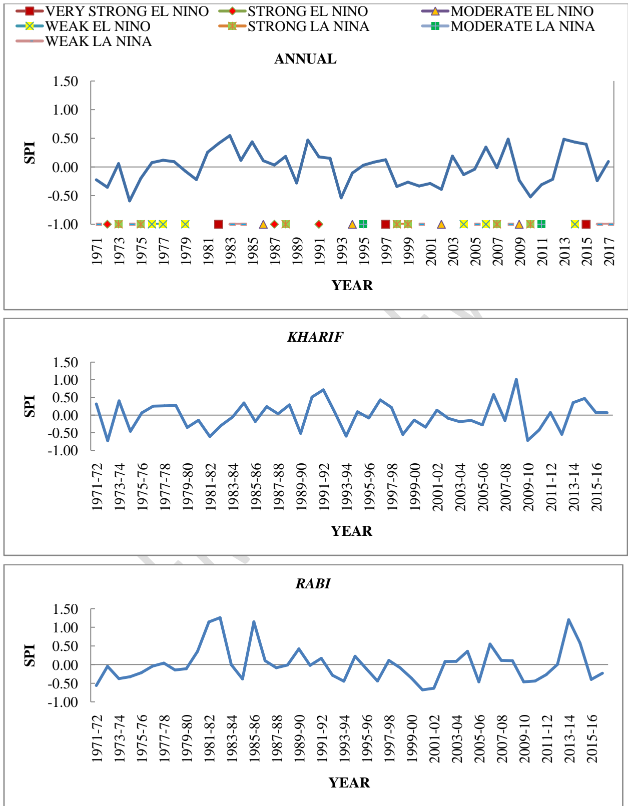
Fig. 1 Standardized precipitation index at Amritsar (Annual, Kharif and Rabi)
