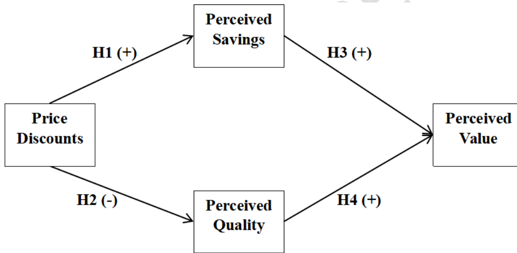
Fig. 1. Framework Model
