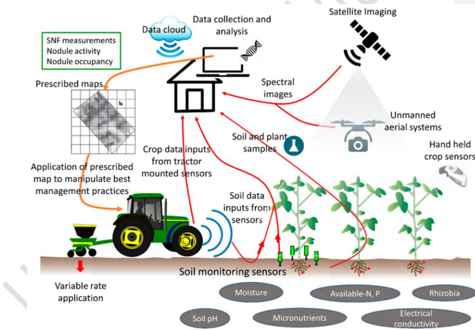
Figure 1. Components of integrated precision horticulture solutions.
