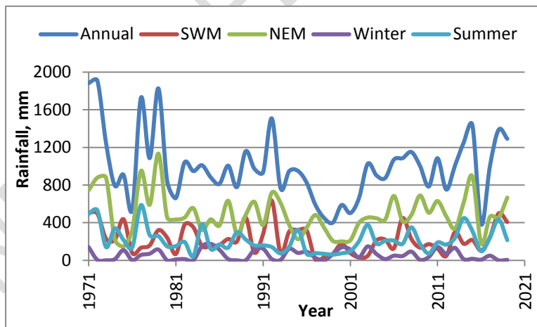
Figure 2. Distribution of seasonal and annual rainfall series of Tenkasi
