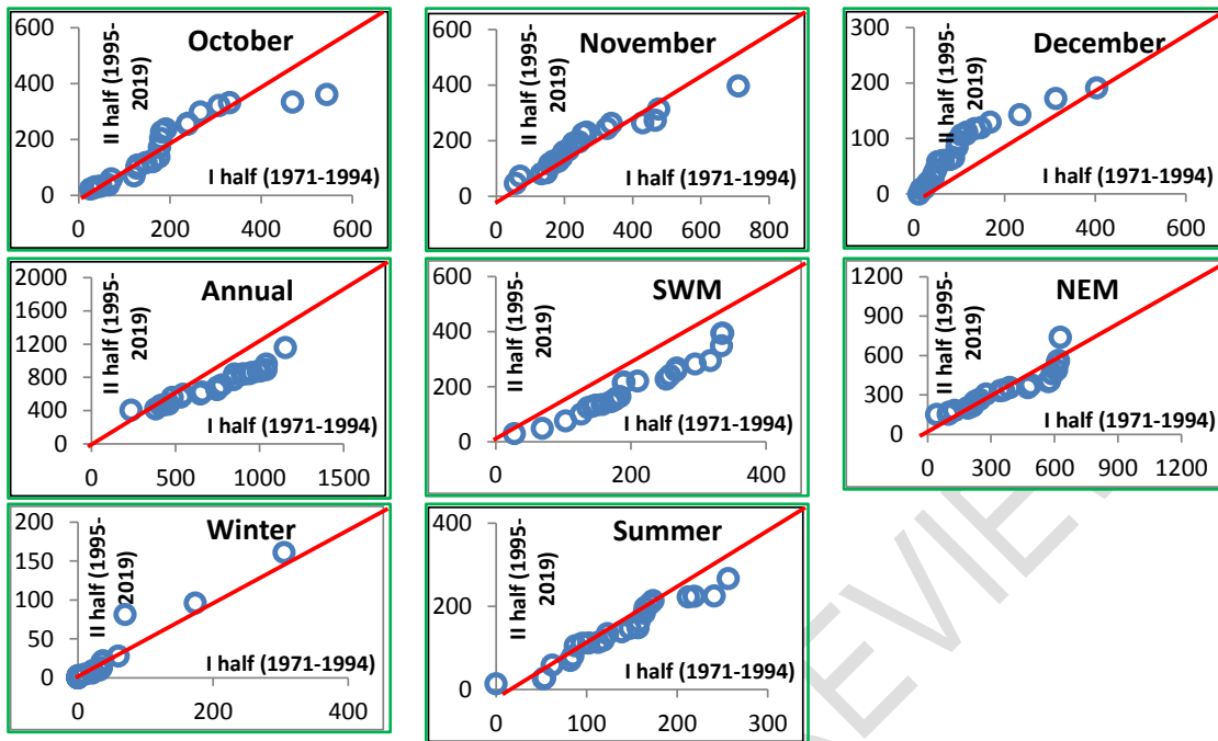
Figure 3. Results of ITA method for different rainfall series of Tenkasi
