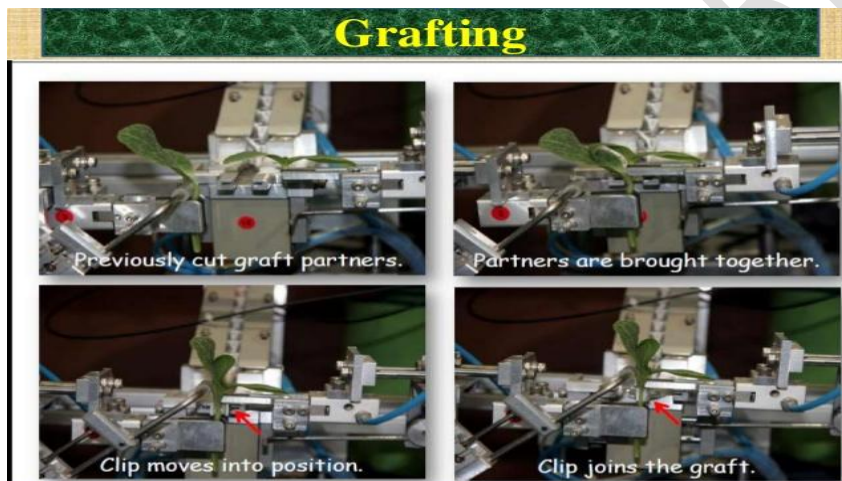
Figure 8. Robotic grafting
