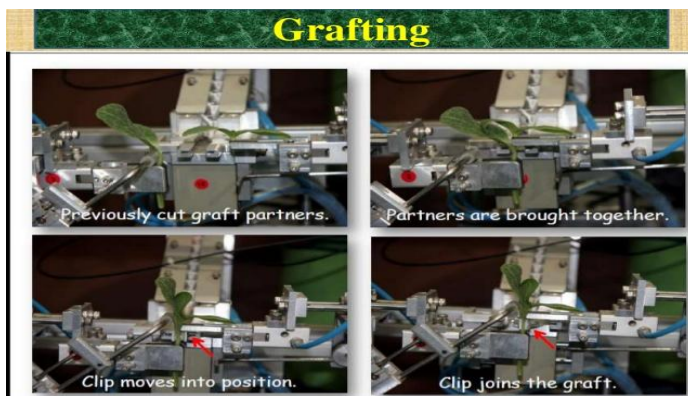
Figure 7. Robotic grafting
