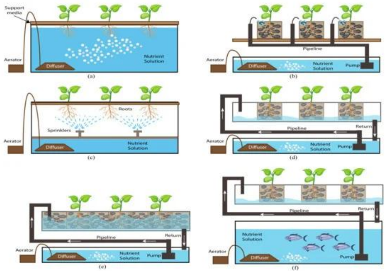
Figure 1. Different types of hydroponic systems. (a) Deep Water Culture. (b) Drip System. (c) Aeroponics. (d) Nutrien Film Technique (NFT). (e) Ebb and flow. (f) Aquaponics
