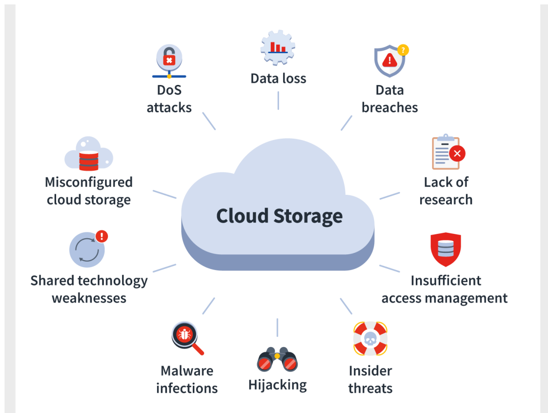
Fig.3.Cloud Security Challenges [19]
