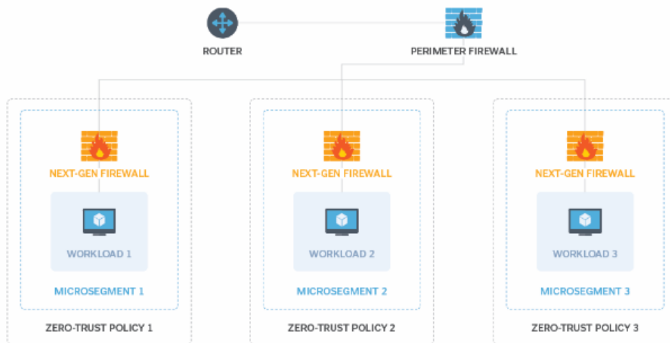
Fig.2.Zero-trust Micro-segmentation [8]
