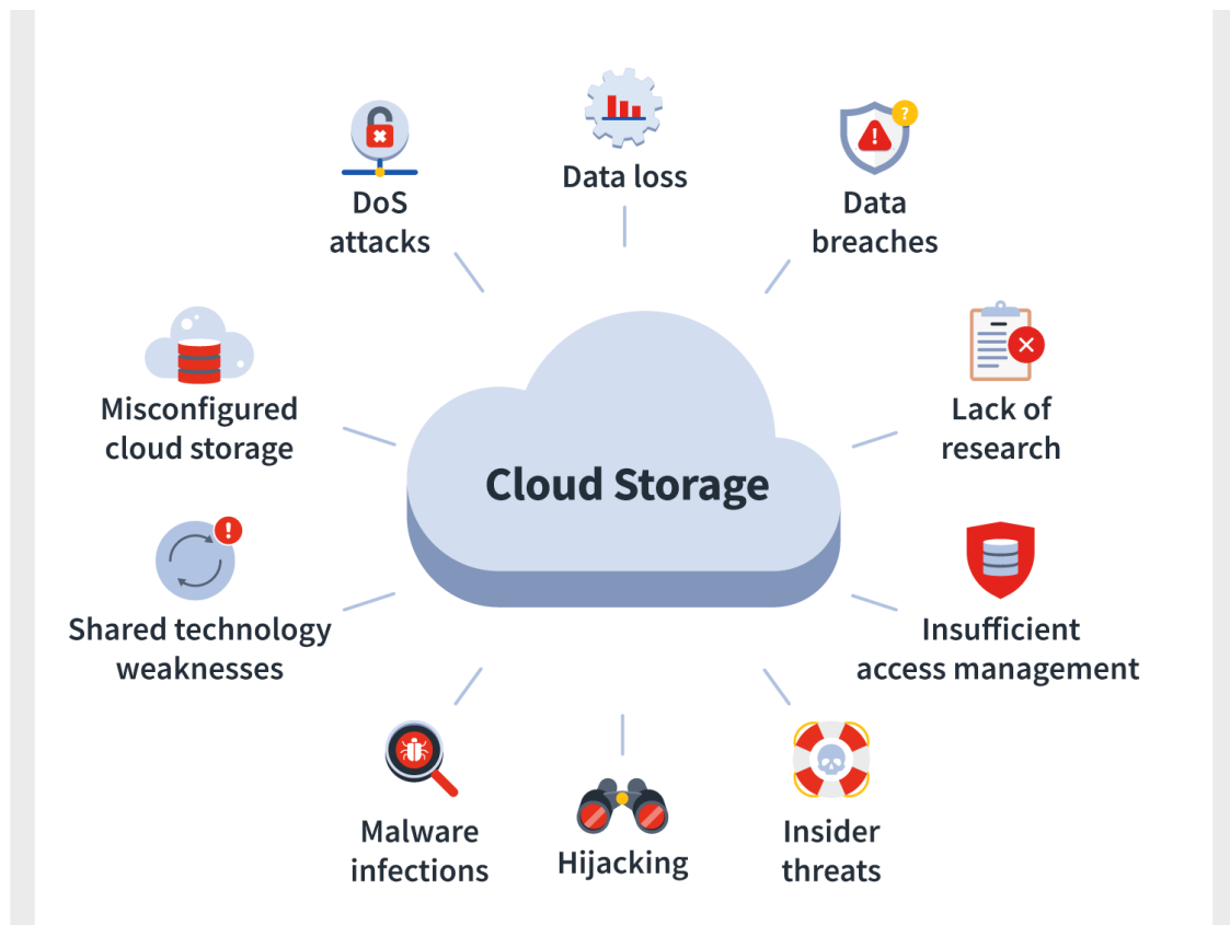
Fig.3.Cloud Security Challenges [18]
