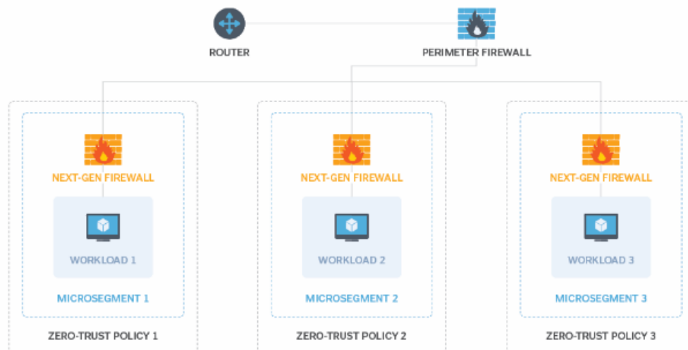
Fig.2.Zero-trust Micro segmentation [8]
