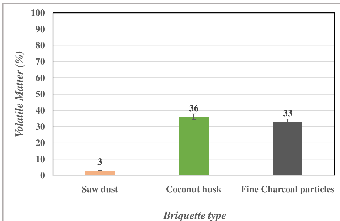
Figure 4: Volatile Matter (%) of briquettes produced from sawdust, coconut husk and fine charcoal particles.
