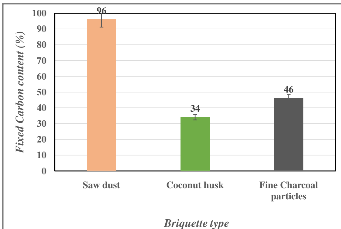
Figure 6: Fixed Carbon contents of briquettes produced from sawdust, coconut husk and fine charcoal particles.
