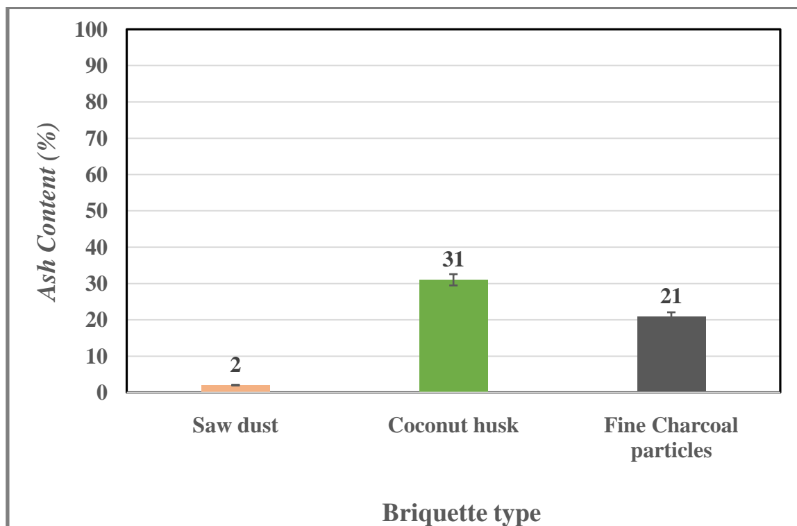
Figure 5: Ash content (%) of briquettes produced from sawdust, coconut husk and fine charcoal particles.
