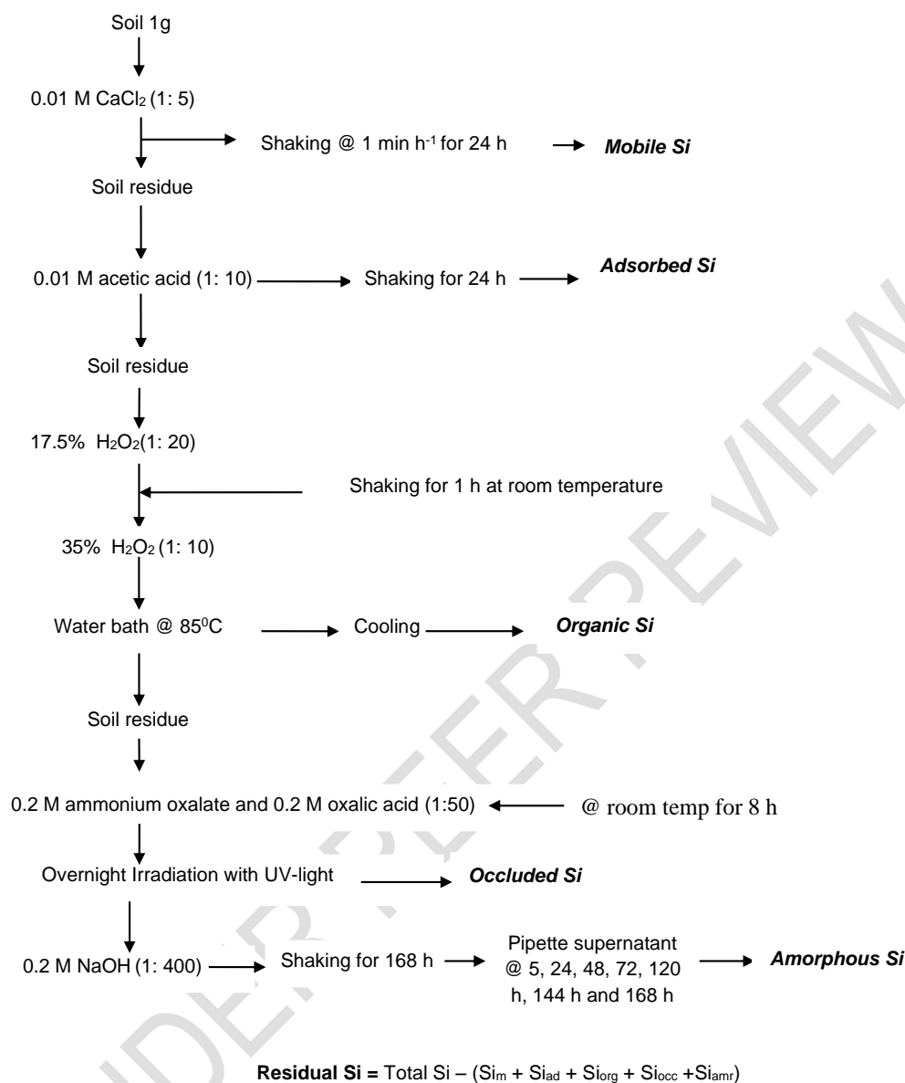
Fig. 2 Flow diagram of fractionation of Si in soil
