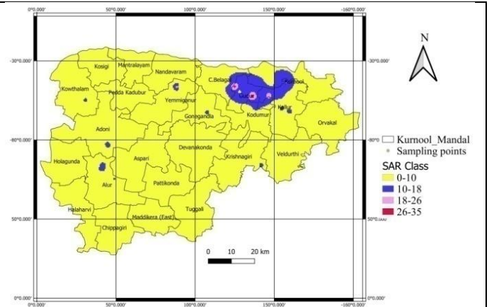
Fig 5. Spatial variability in SAR of groundwater
