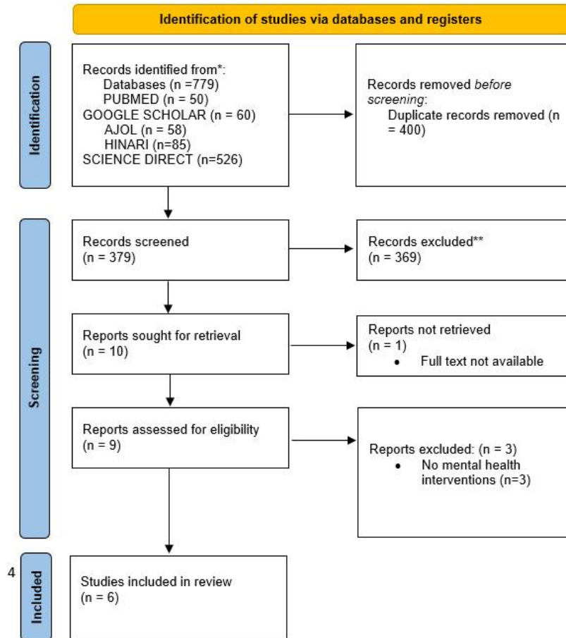
Figure 1: PRISMA CHART
