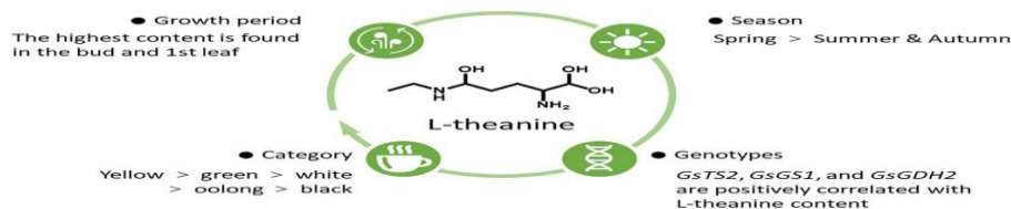
Figure: 3. Influencing factors of L-theanine Theanine content in tea leaves (24).
