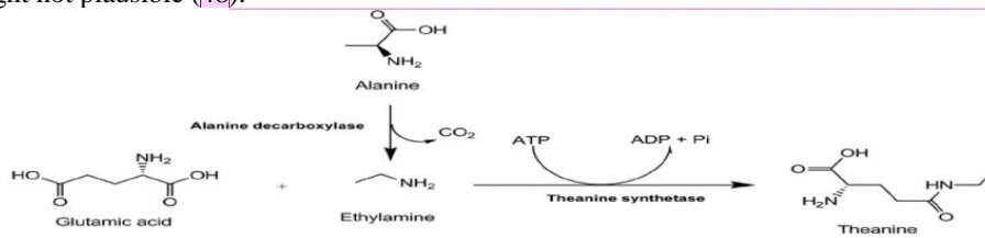
Figure 2. Theanine synthesis from glutamic acid and ethylamine. Ethylamine formation from alanine is also shown (34).
