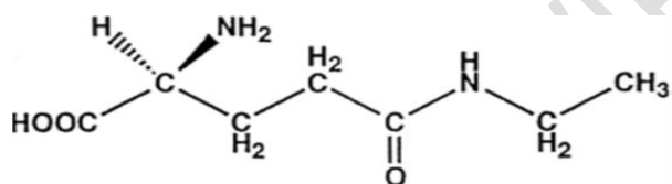
Figure 1. Chemical structure of L-Theanine (47).
