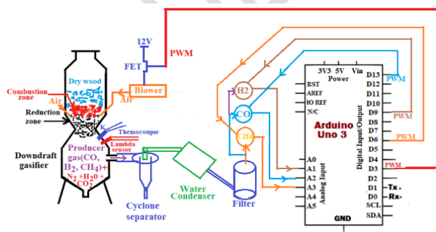
Figure 6 : MQ gas sensors PWM drivers overview
