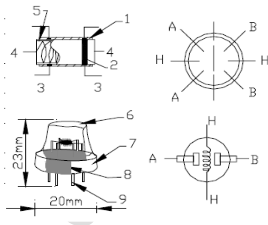
Figure 1 :MQ gas sensors structure
