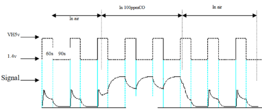
Figure 5 : Heating cycle requirement for MQ sensors [25]
