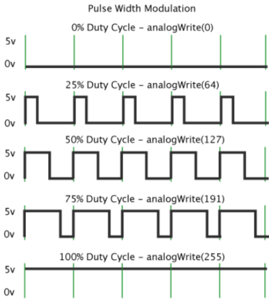
Figure 4 : PWM examples in Arduino [24]
