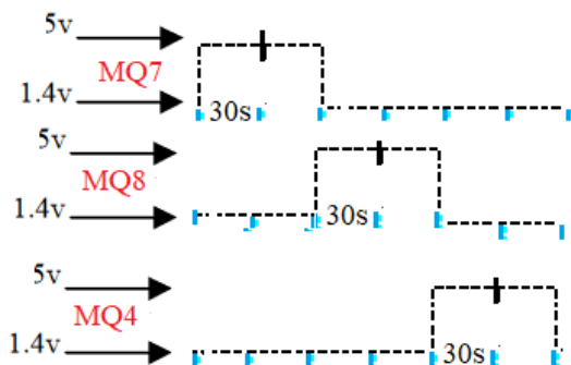
Figure 6 : MQ gas sensors PWM drivers overview
