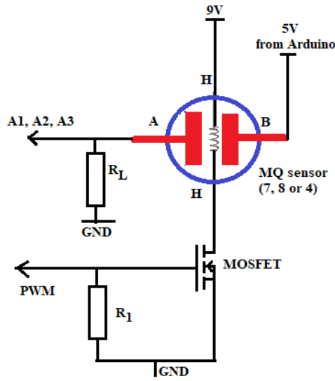
Figure 2 : PWM heating circuit for a MQ sensor
