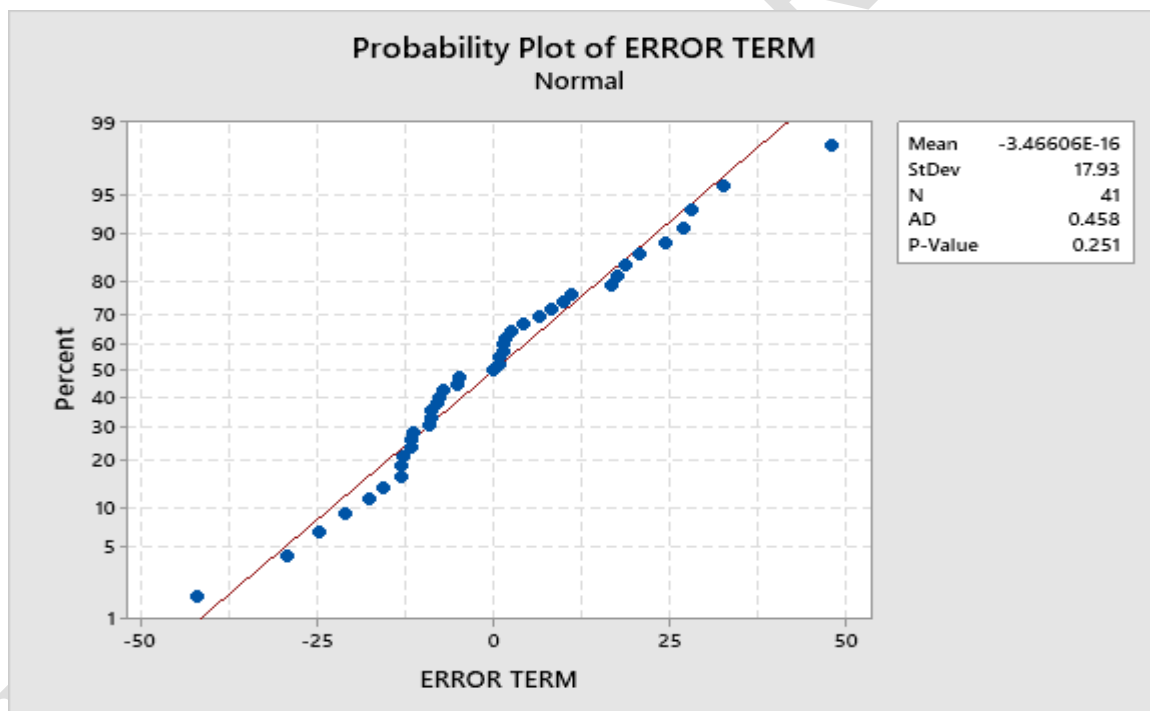
Fig. 2. The Anderson-Darling Test for Normality Assumption
