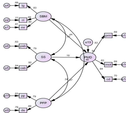
Figure 1. Structural Equation Model 3 in Standardized Solution
