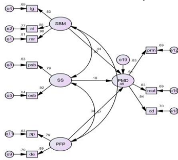
Figure 1. Structural Equation Model 3 in Standardized Solution
