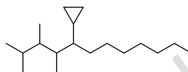
(2,3,4-triethyl)dodecan-5-yl)cyclopane
