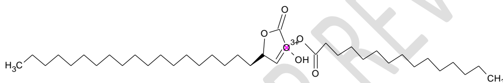
Ascorbic acid, 2,6-dihexadecanoic acid
