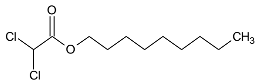
nonyl 2,2-dichloroacetate
