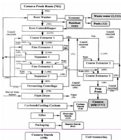
FIGURE 2, Diagram for Cassava Starch Extraction
