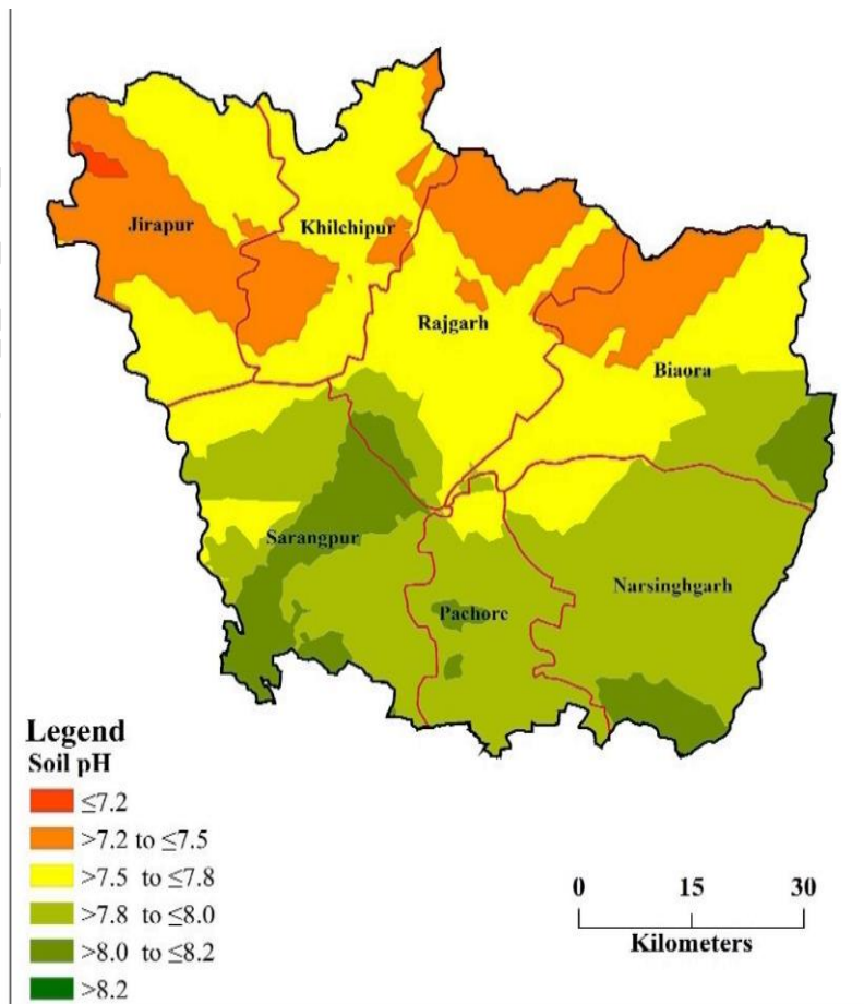
Figure 2: Semi-Ordinary kriging model (A) pH (B) Soil EC organic carbon
