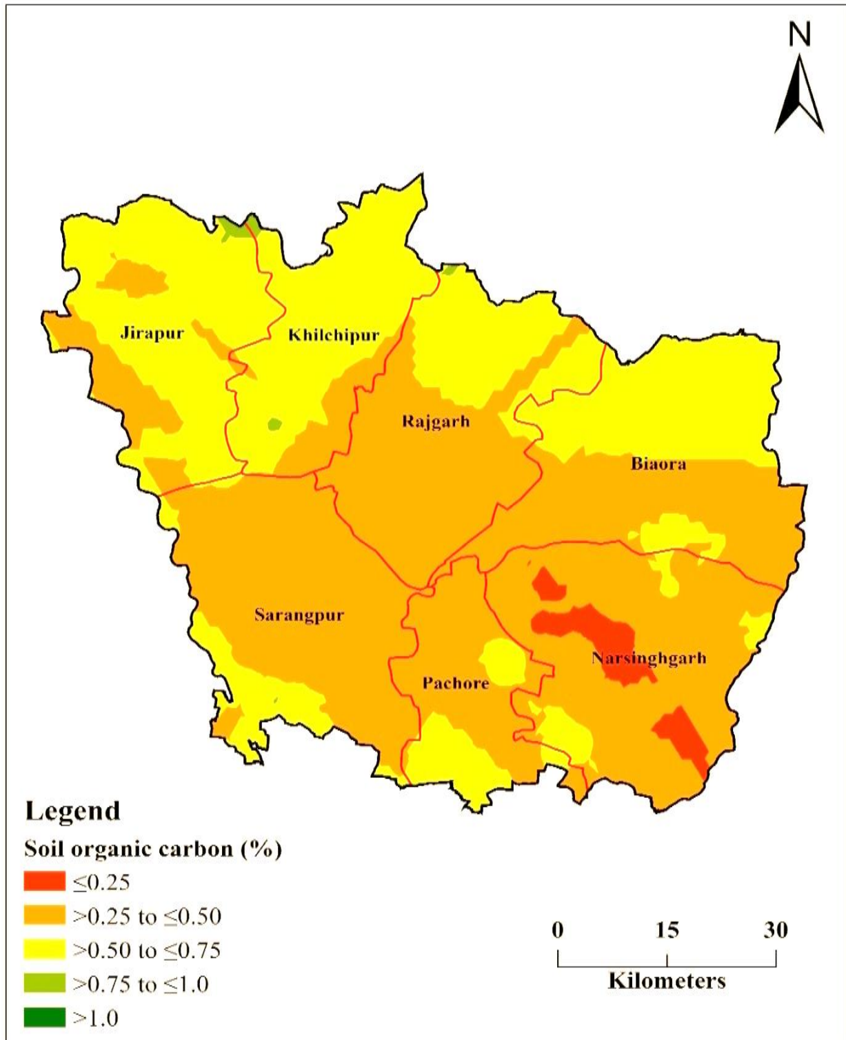
Figure 5: Map of Soil organic carbon (0-20 cm) with best-fitted model (Ordinary kriging; exponential)
