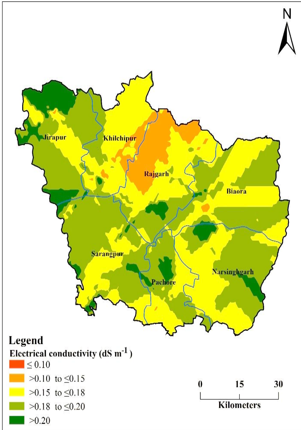
Figure 4: Map of Soil EC ( \text{dS m}^{-1} ) (0-20 cm) with best-fitted model (Ordinary kriging; exponential)
