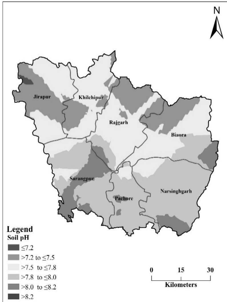
Figure 3: Map of Soil pH (0-20 cm) with best fitted model (Ordinary kriging; exponential)
