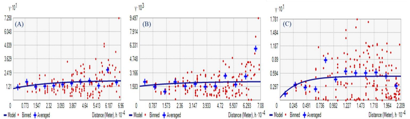
Figure 2: Semi-variogram of Ordinary kriging best-fitted model (exponential) (A) pH (B) Soil EC (C) Soil organic carbon
