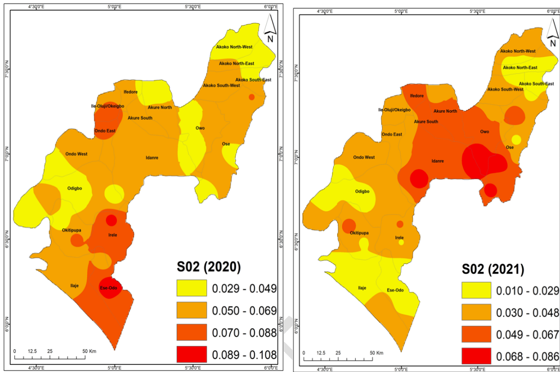
Figure 4 (a) SO 2 2020
