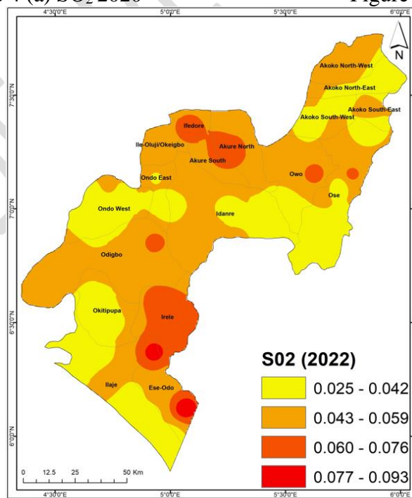
Figure 4 (c) SO 2 2022
