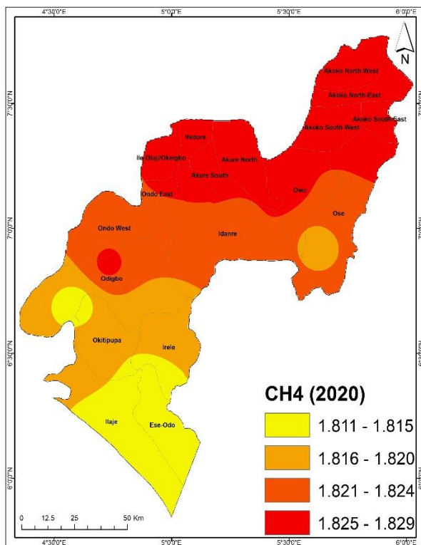
Figure 1 (a) CH 4 2020
