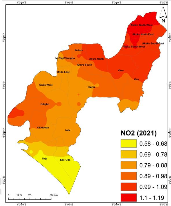
Figure 3 (b) NO 2 2021
