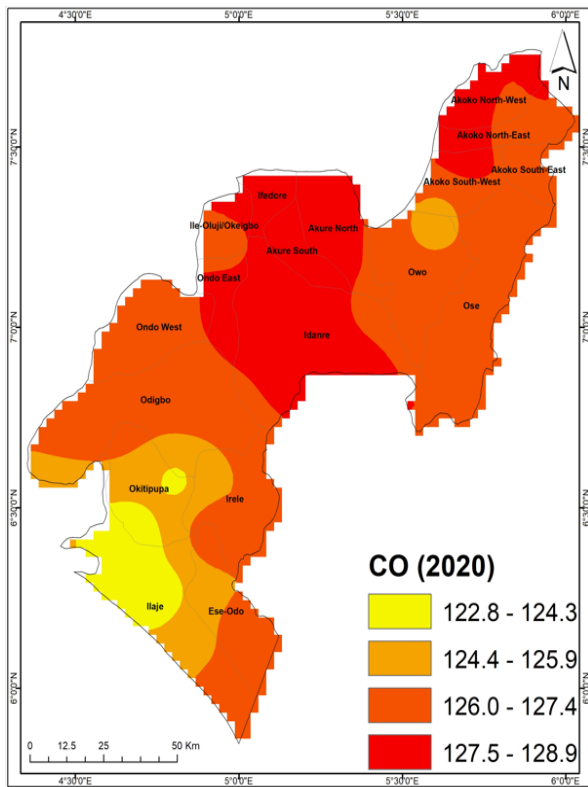
Figure 2 (a) CO 2020
