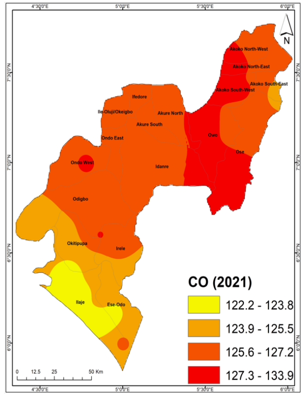
Figure 2 (b) CO 2021
