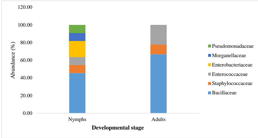
Fig. 5. Bacterial abundance of nymphs and adults of B. tabaci at family level
