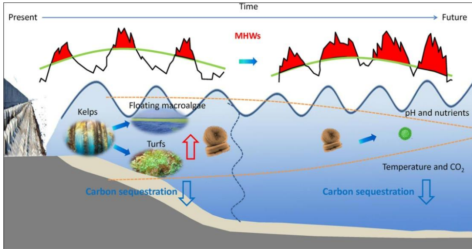
Fig. 3. Comparative effects of normal and heatwave conditions in oceans (Source: IITM, Pune)
