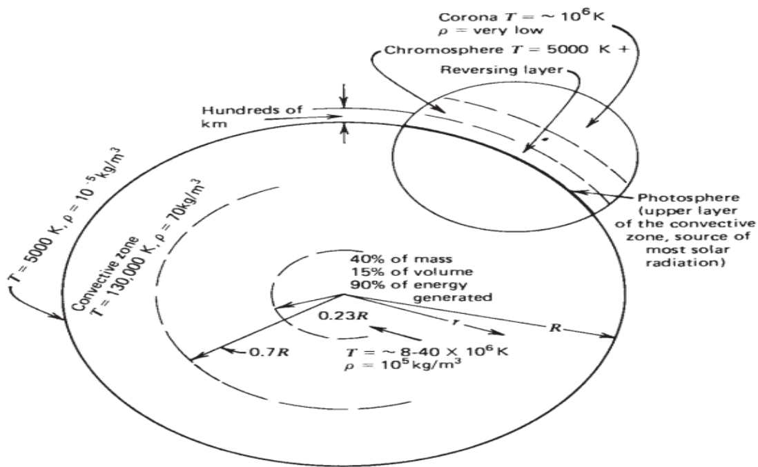
Figure 1: The structure of the sun [7]
