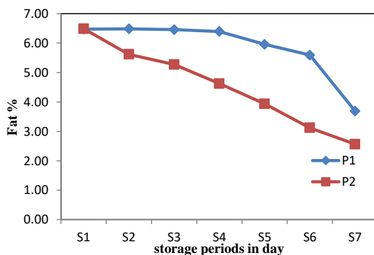
Fig. 5 Effect of packaging material and storage duration on fat content of multigrain mixes from finger millet malt and moth bean malt.
