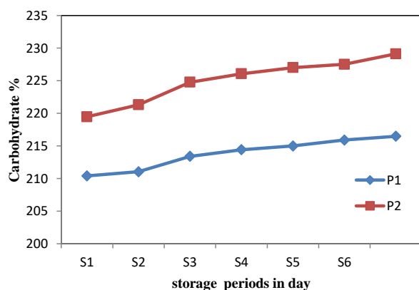
Fig. 8 Effect of packaging material and storage duration on carbohydrate content of multigrain mixes from finger millet malt and moth bean malt.
