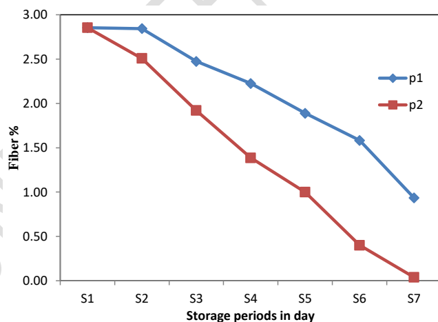
Fig. 6 Effect of packaging material and storage duration on fiber content of multigrain mixes from finger millet malt and moth bean malt.
