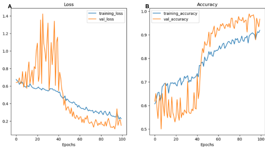
Fig. 4: Model accuracy and loss curves
