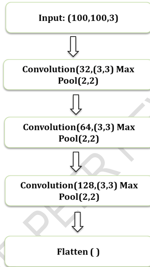
Fig. 1. CNN architecture used in the study
