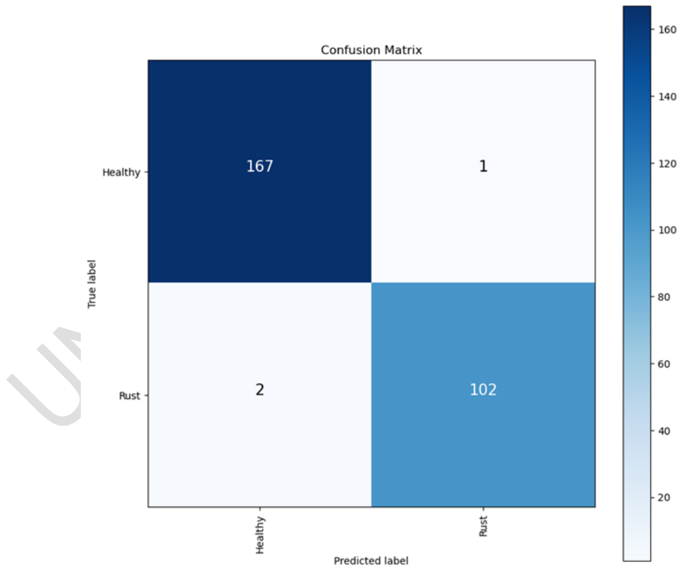
Fig. 6: Confusion matrix for the developed model
