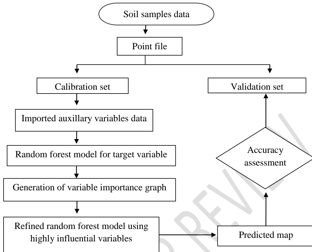
Fig. 4. Flow chart of Random forest model
