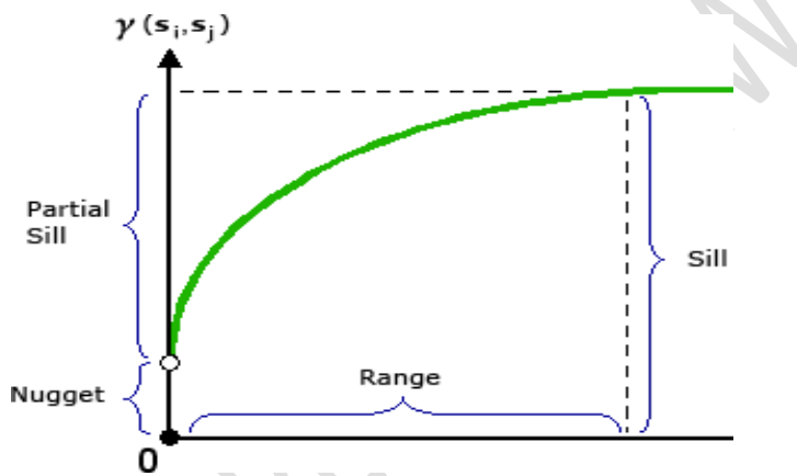
Fig. 2. Component of semivariogram model
