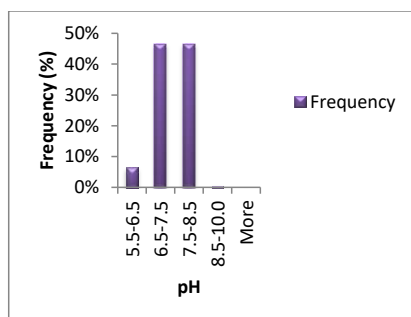
Fig. 5. Soil pH
