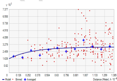
Fig. 7. Exponential model of soil pH
