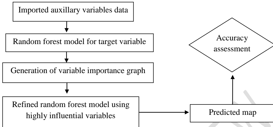
Fig. 4. Flow chart of Random forest model
