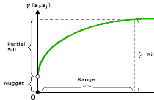
Fig. 2. Component of semivariogram model
