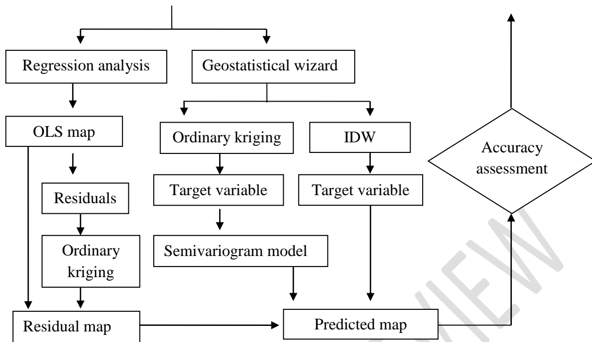
Fig. 3. Flow chart of Geostatistical analysis
