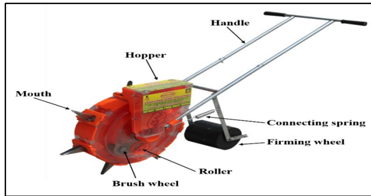
Fig. 1: View of manual seeder
