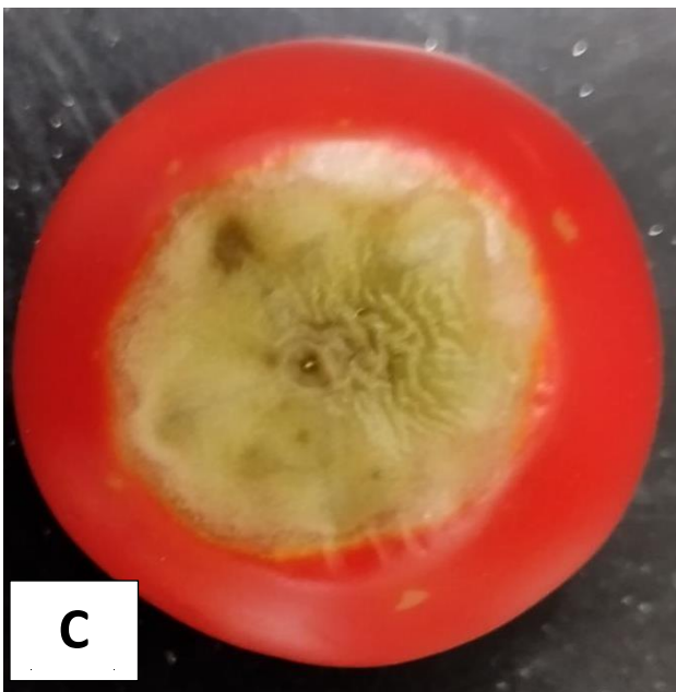
Fig.2: Physiological parameters of tomato fruits. A-C: Symptoms of blossom end rot; B-D: PRANAM Ca sprayed healthy fruits
