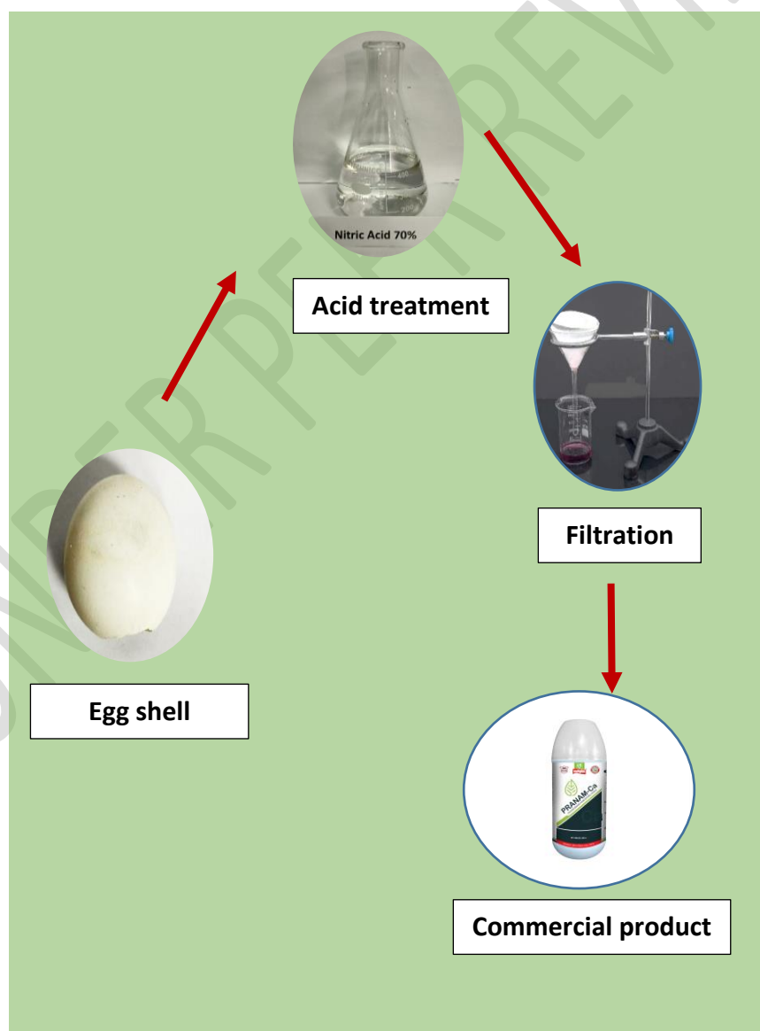
Fig.1: Preparation of PRANAM Ca
