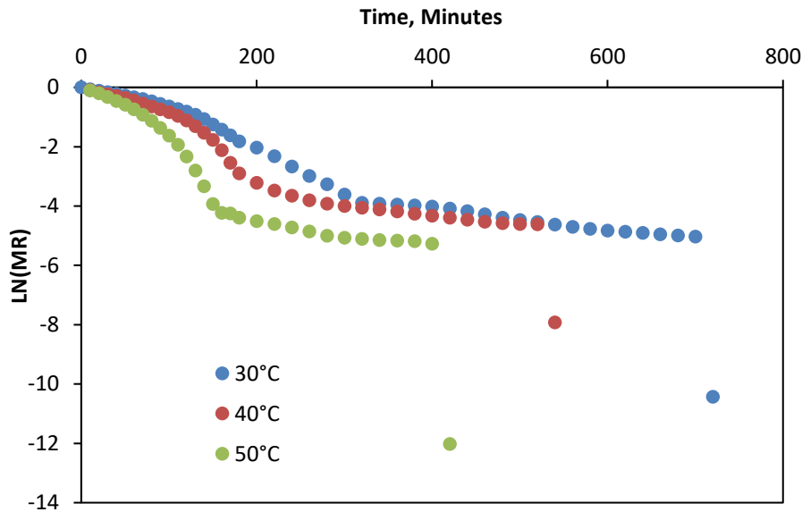
Fig. 4 Plot Ln(MR) of Drum Stick Leaf Powder
