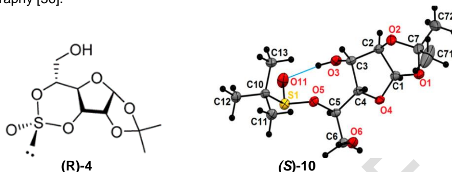
Fig. 8. ( R )-1,2- O -isopropylidene-3,5- O -sulfinyl- \alpha -D-glucopyranose ( R )-4 and molecular structure of ( S )-1,2- O -isopropylidene-(5- O - \alpha -D-glucopyranosyl) t -butanesulfinate 10.
