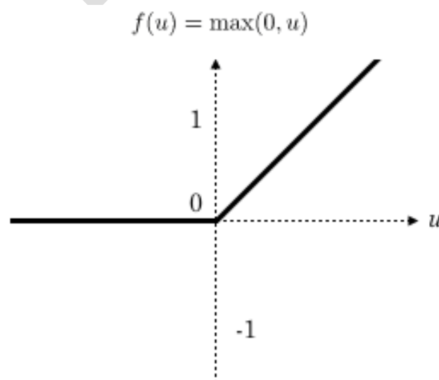
fig. 3. ReLU function appearance [n]
