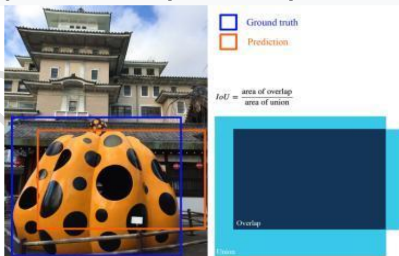
fig. 5. IoU illustration [p]
