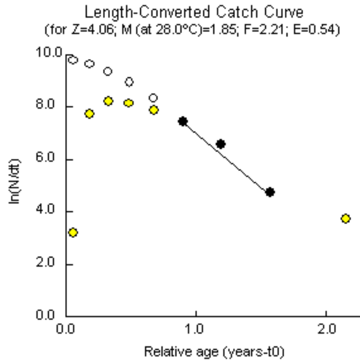
Figure 4. Length-converted catch curve of Gudusia chapra for estimation of total mortality
