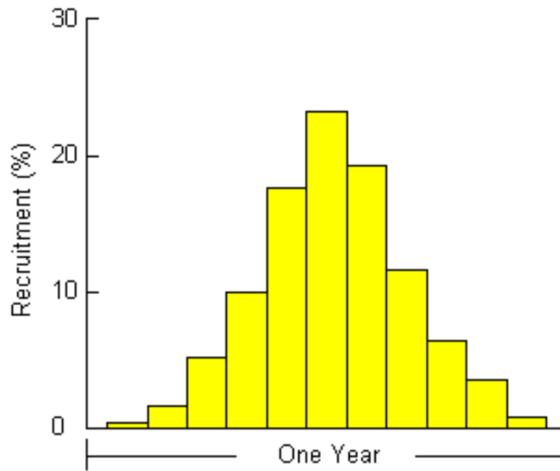
Figure 5. Recruitment pattern of Gudusia chapra
