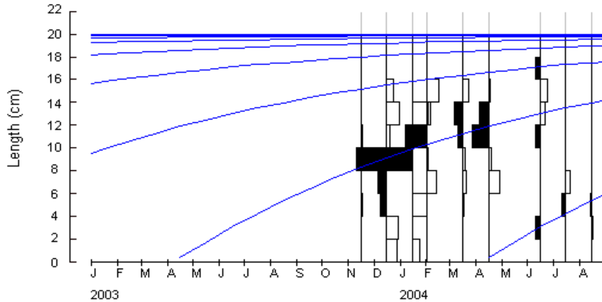
Figure 2. Von Bertalanffy growth function plot and length frequencies of Gudusia chapra [Asymptotic length ( L_{\infty} ) = 19.95 cm, & VBGF growth constant (K) = 0.89]
