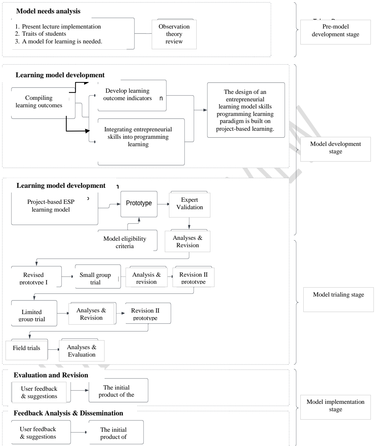
Fig. 1. Research Procedure
