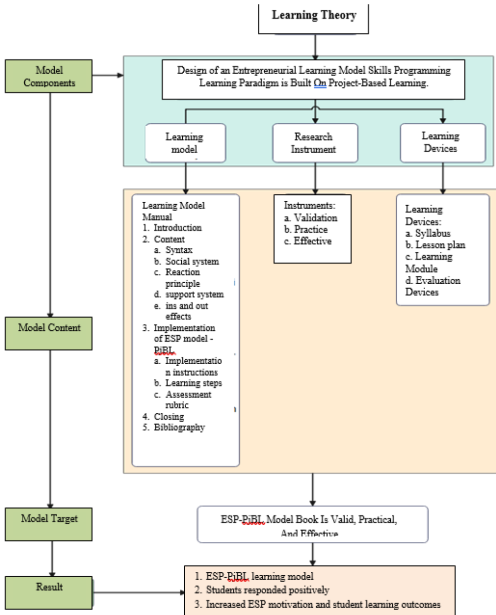
Fig. 6. Learning Theory
