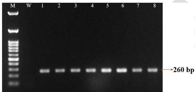
Fig.3. Amplification of Fusarium isolates with Fusarium oxysporum f. sp. cubense specific primer developed by Carvalhais et al. , (2019). Lane M: 100bp ladder, Lane W: Negative control, Lane 1-8: Foc S-6, S-32G, S-35, S-39, S-53, S-56, S-63, S-67 respectively.
