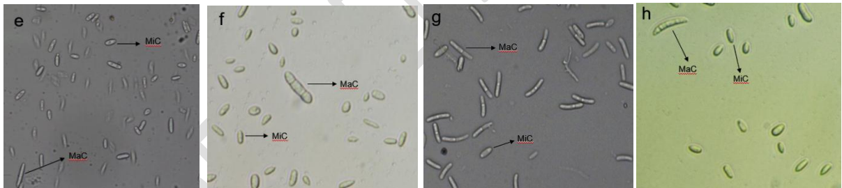
E,F,G,H - colony appearance of Foc isolates S35, S39, S53 and S63 respectively; e, f, g, h - microscopic spore image of Foc isolates S35, S39, S53 and S63 respectively; MiC – microconidia; MaC – macroconidia
