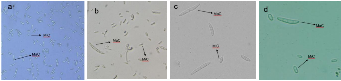
A,B,C,D – colony appearance of Foc isolates S6, S32G, S56 and S67 respectively; a,b,c,d – Microscopic spore image of Foc isolates S6, S32G, S56 and S67 respectively; MiC – microconidia; MaC – macroconidia
