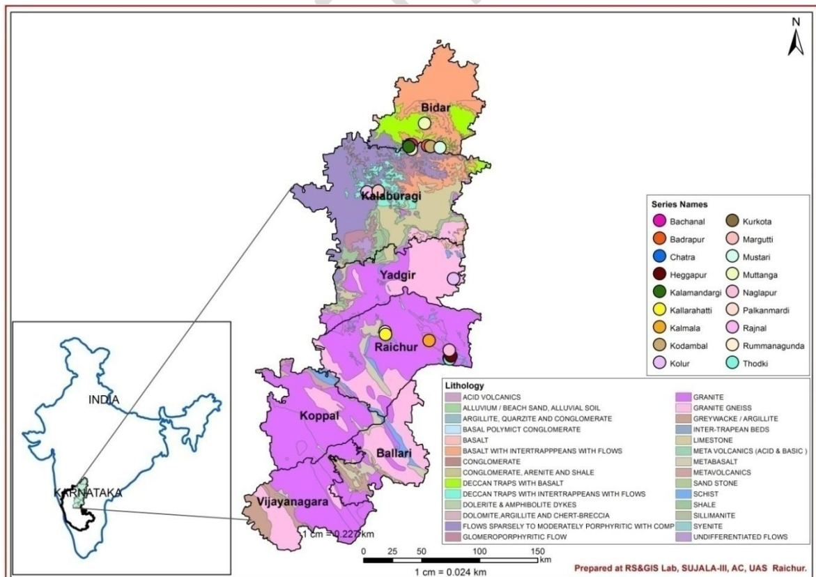
Fig. 2: Geology map of soil profile sampling sites of the soils series
