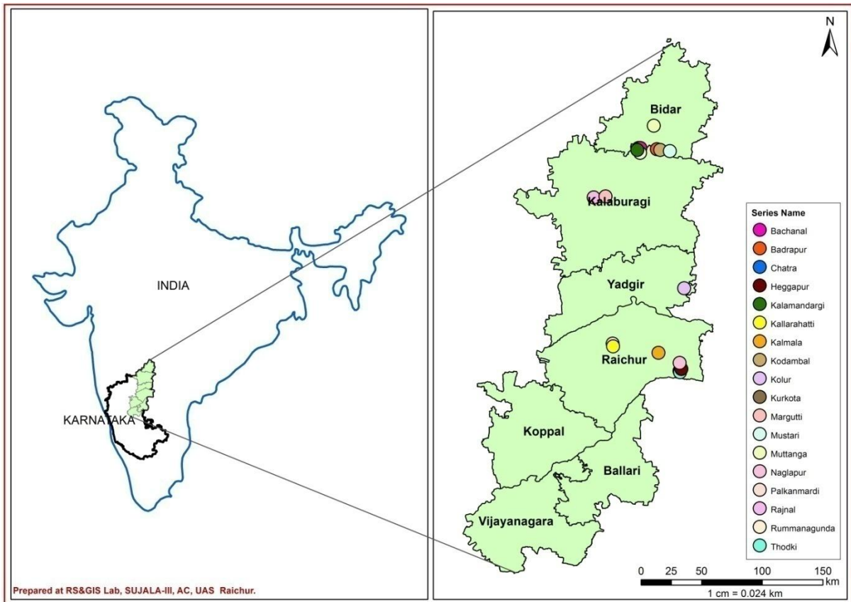
Fig. 1: Location map of soil profile sampling sites of the soils series
